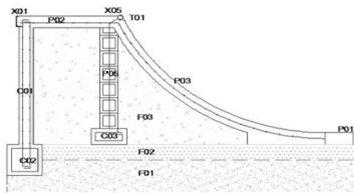
Detalle Quarter
